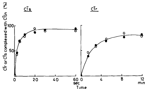
Fig 1 Comparison of the rates of reaction of iodinated and non-iodinated C 1 r and C 1 s with C 1 In. 125 I-labelled C 1 r or C 1 s were diluted with cold C 1 r or C 1 s such that the overall labelling represented 5 atoms I/100 molecules C 1 r or C 1 s. The C 1 r (450 \mu g/ml) or C 1 s (440 \mu g/ml) in 5 mM triethanolamine–HCl, 145 mM NaCl, 5 mM EDTA (pH 7.4) was then incubated with C 1 In (920 \mu g/ml) at 37°C. Reaction was stopped at various times by placing 50 \mu l of the reaction mixture in 50 \mu l 0.2 M Tris–HCl, 8 M urea, 2% w/v SDS, 40 mM iodoacetamide (pH 8.0) and incubating 4 min at 100°C. Samples were then examined on SDS–polyacrylamide gels, and the gels stained and scanned. The rate of uptake of total (i.e., labelled + unlabelled C 1 r or C 1 s into complexes with C 1 In (●) was estimated from the decrease in intensity of the free C 1 r or C 1 s peaks on the gels. Gels were then sliced and the rate of complexation of labelled C 1 r or C 1 s with C 1 In (○) calculated from the radioactivity associated with the free protease and C 1 In–protease complex bands.
